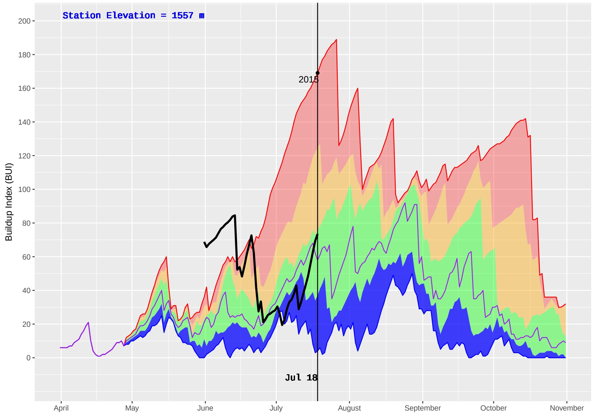
SKOONKA (1024) : Historical (2008–2016) and Current (2018) Daily Buildup Index (BUI)
