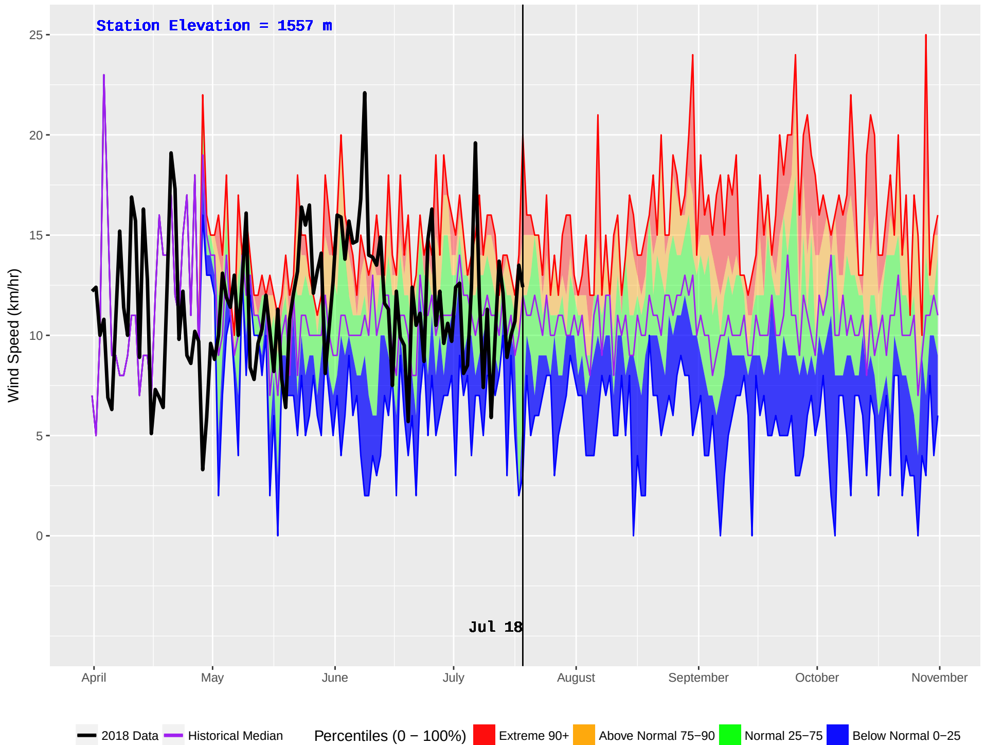
SKOONKA (1024) : Historical (2008–2016) and Current (2018) Daily Wind Speed
