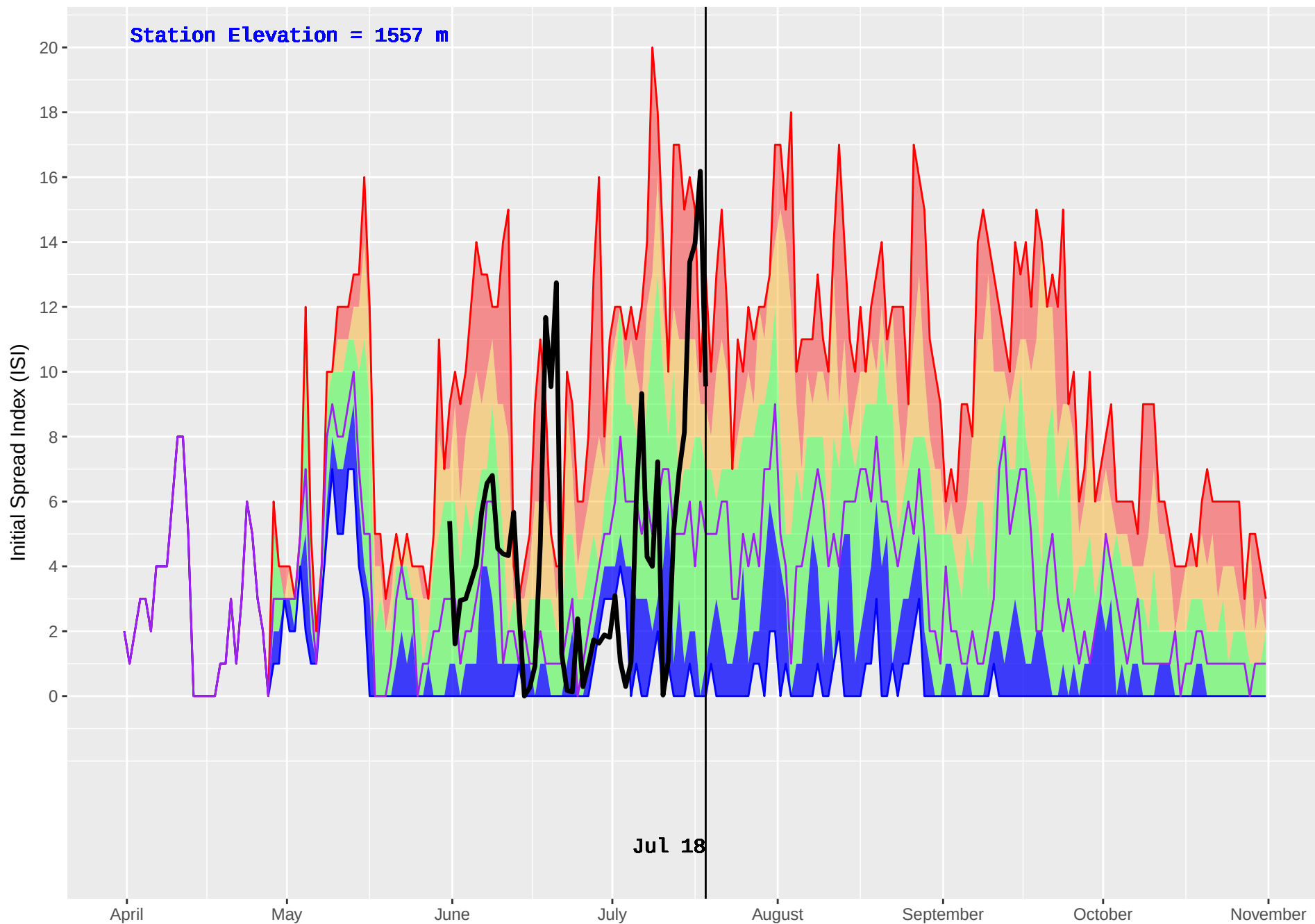
SKOONKA (1024) : Historical (2008–2016) and Current (2018) Daily Initial Spread Index (ISI)
