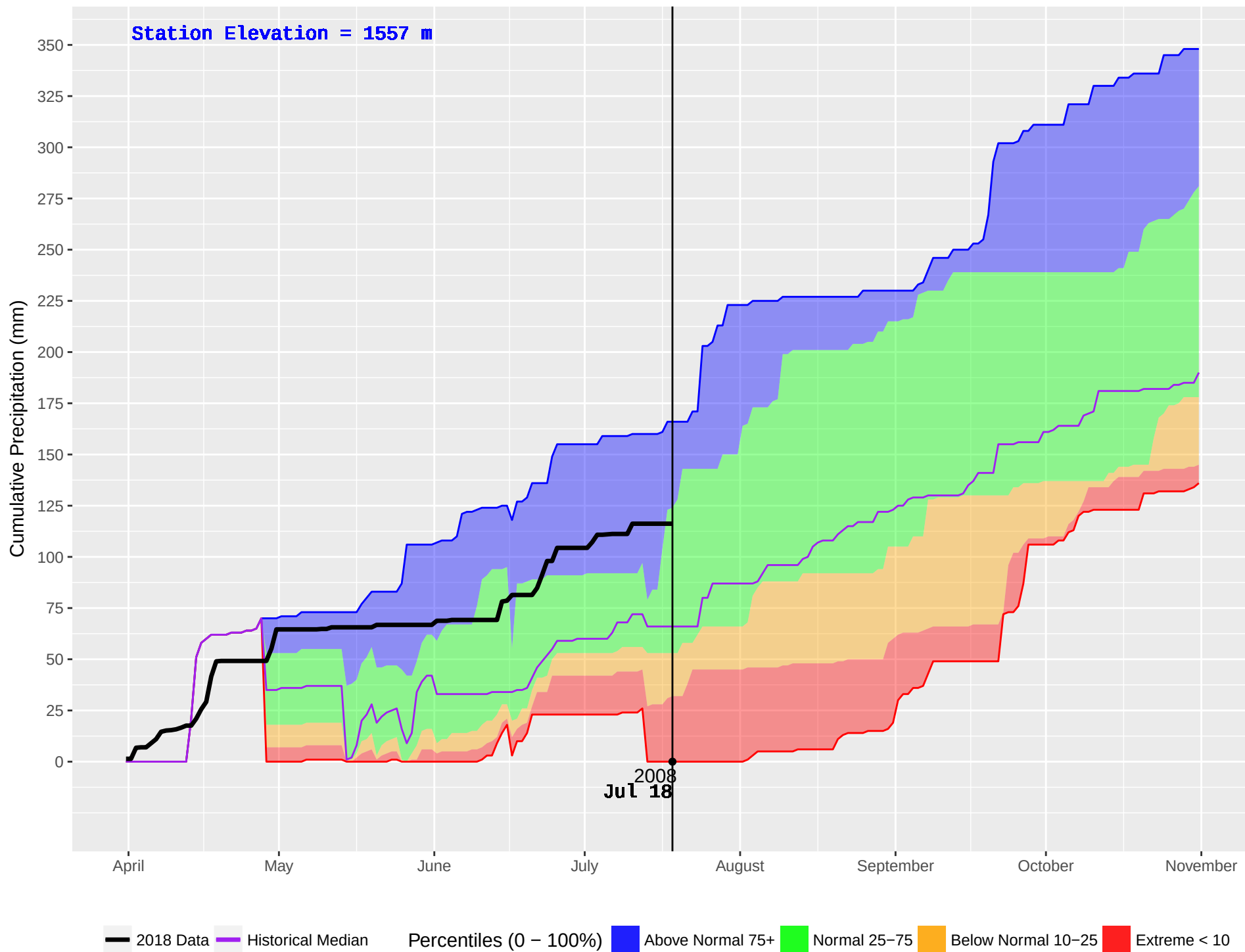
SKOONKA (1024) : Historical (2008–2016) and Current (2018) Daily Cumulative Precipitation
