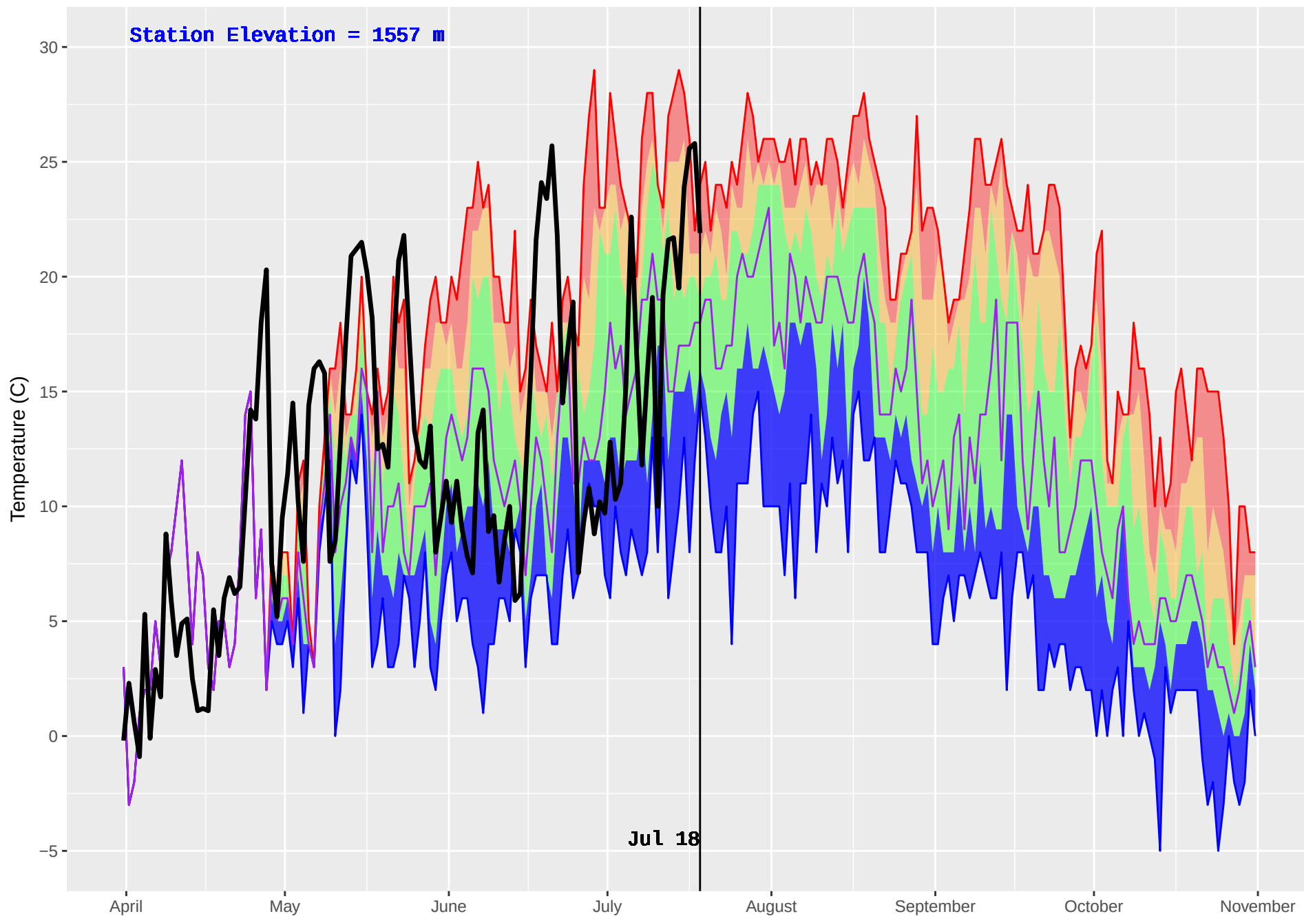
SKOONKA (1024) : Historical (2008–2016) and Current (2018) Daily Temperature
